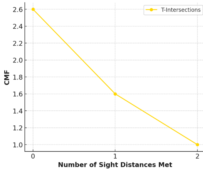
Figure 40. CMF Plot for T-Intersection (Speed Limit \leq 25 mph) Based on Number of Sight Distances Met. CMF = crash modification factor.
