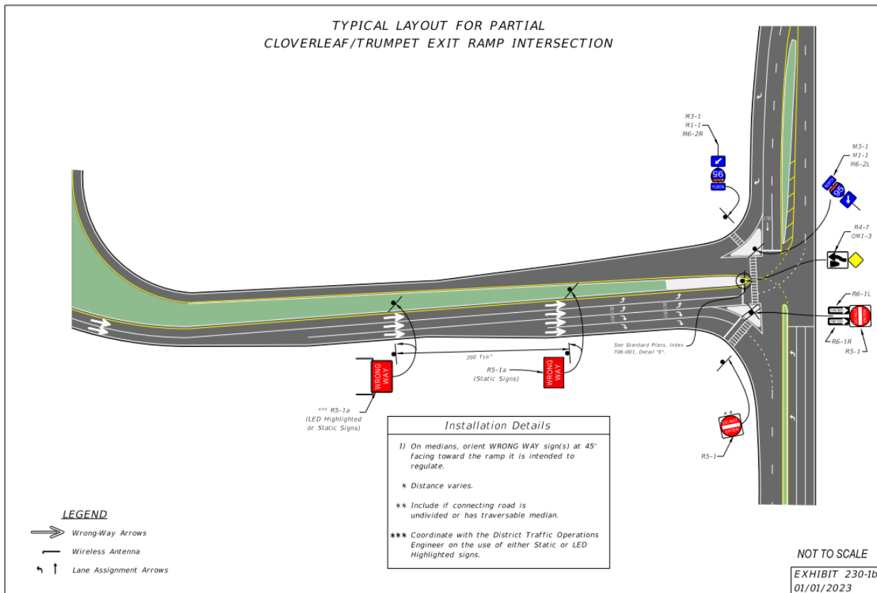
Figure 35. FDOT Typical Layout for Wrong-Way Driving Detection System Signing and Markings (FDOT Design Manual, 2023). Used with permission.
