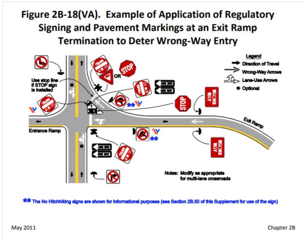
Figure B3. VA Supplement MUTCD Example for Wrong-Way Driving Sign at Exit Ramp
