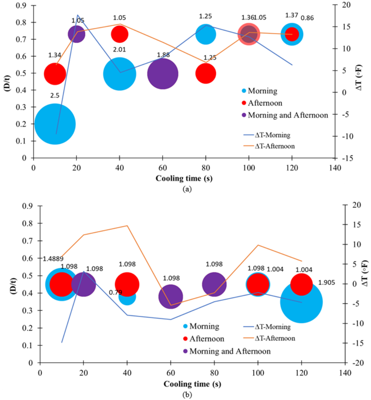
Figure 37. Characterization of the defects detected when the heating time was 20 seconds (a) east side and (b) west side (values next to each bubble represent the aspect ratio [AR]) (ideal case is when a smaller AR with a higher defect depth to wall thickness ratio [D/t] has been detected)
