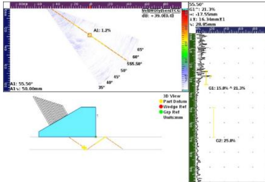
Figure 46. An example of less confident signal return (note: 1 mm = 0.039 in)
