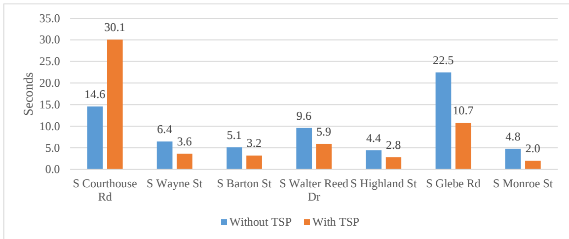
Figure 11. Overall Stop Delay for Buses, Arlington Simulation Results
