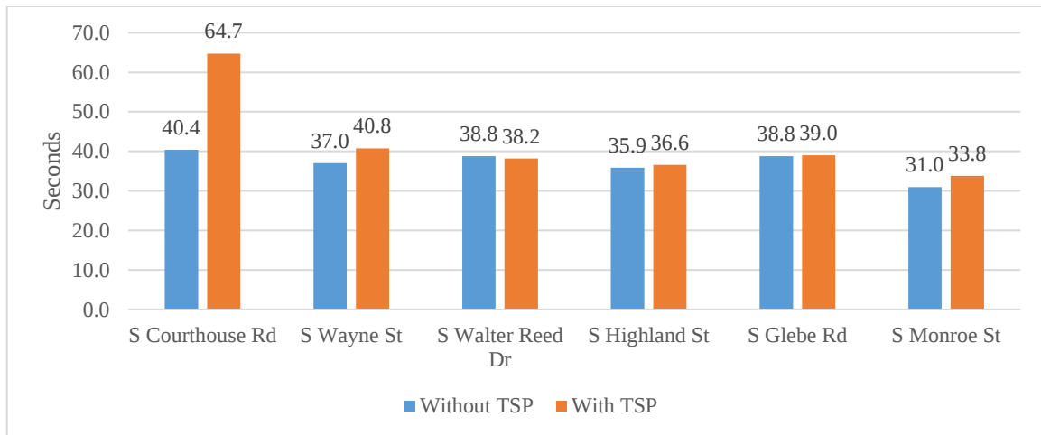
Figure 12. Pedestrian Delay, Arlington Simulation Results
