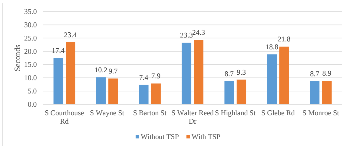
Figure 10. All-Vehicle Stop Delay, Arlington Simulation Results
