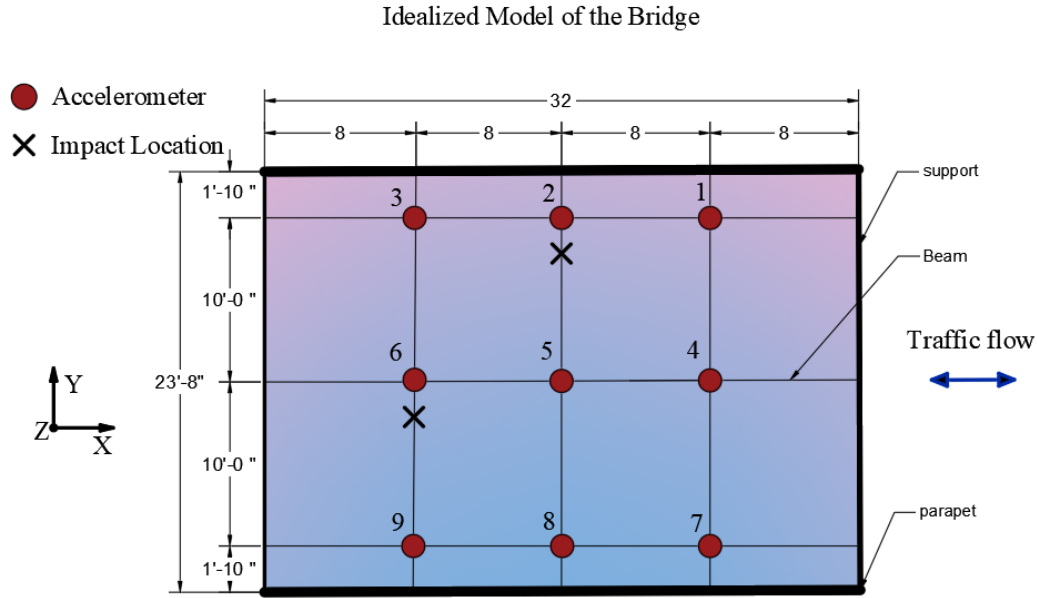
Figure 17 – Instrumentation Configuration for Brattons Creek Bridge for Vibration Testing
