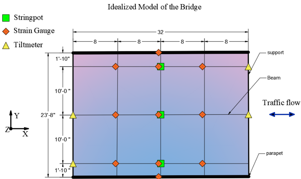
Figure 12 – Instrumentation Configuration for Brattons Creek Bridge for Live Load Testing
