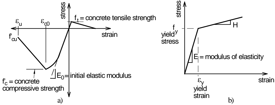
Figure 42. Uniaxial Material Laws used in Beam Models: a) Hognestad Concrete Material Model (Hesham and Mohd, 1994) and b) Elastoplastic Material Model with Linear Kinematic Hardening for Strands
