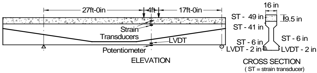
Figure 34. Test 3, Iteration 1 Loading Arrangement and Instrumentation Layout
