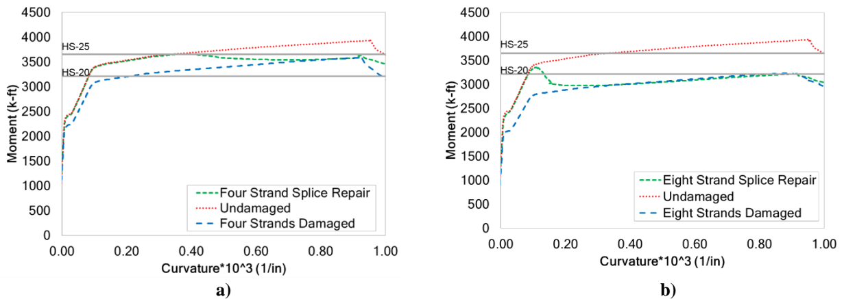
Figure 74. Moment-Curvature Response of Prototype Girder Investigating the Effect of Strand Splice Repair: a) Splice Repair on 4 Strands and b) Splice Repair on 8 Strands
