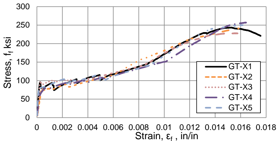
Figure 50. Stress vs. Strain Behavior of Single-Ply Direct Tension Tests
