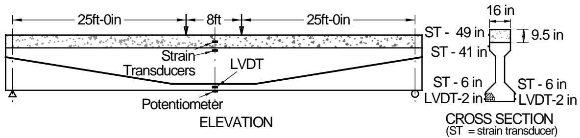
Figure 33. Test 2 Loading Arrangement and Instrumentation Layout
