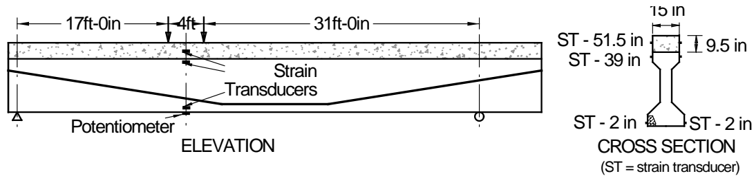
Figure 38. Test 5 Loading Arrangement and Instrumentation Layout
