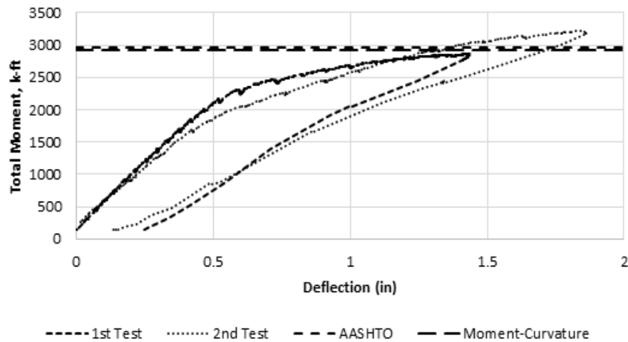
Figure 52. Test 1 Moment Versus Deflection Behavior
