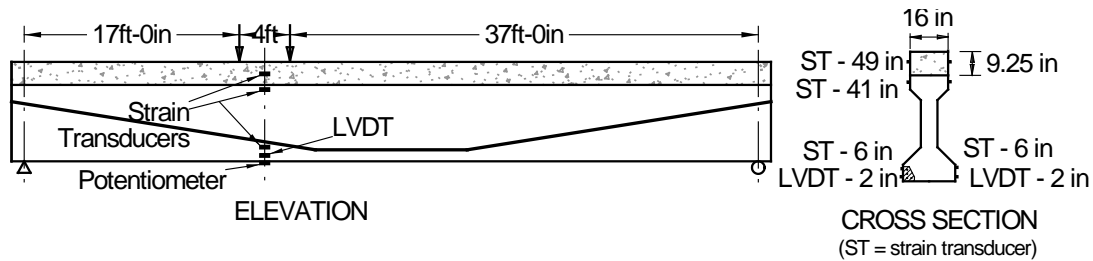
Figure 36. Test 4, Iteration 1 Loading Arrangement and Instrumentation Layout
