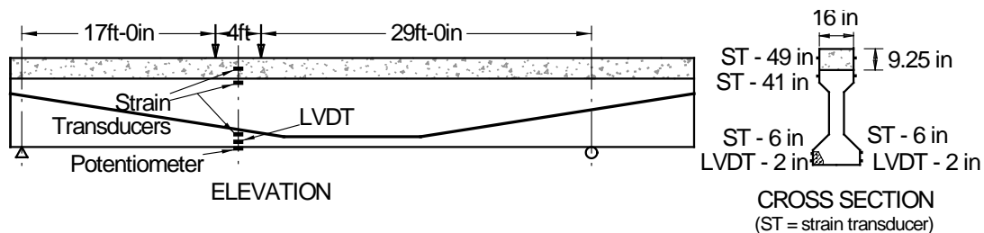
Figure 37. Test 4, Iteration 2 Loading Arrangement and Instrumentation Layout
