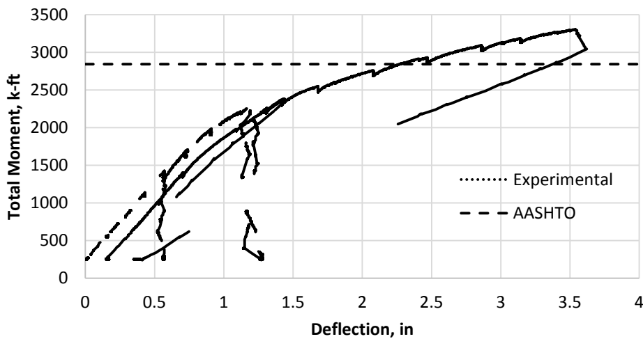
Figure 61. Test 6 Moment Versus Deflection Behavior
