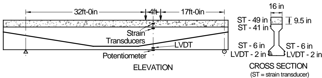
Figure 35. Test 3, Iteration 2 Loading Arrangement and Instrumentation Layout
