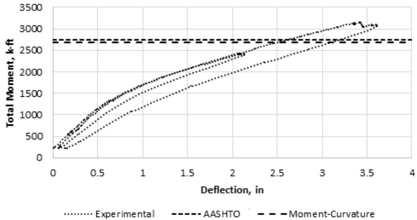
Figure 58. Test 4, Iteration 2 Moment Deflection Behavior
