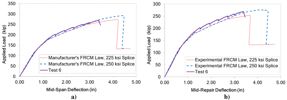
Figure 66. Comparison of Experimental and Analytical Load-Deflection Curves for Test 6: a) FRCM Model Based on Manufacturer’s Data (Man.), b) FRCM Model Based on Experimental Material Test Data (Exp.)
