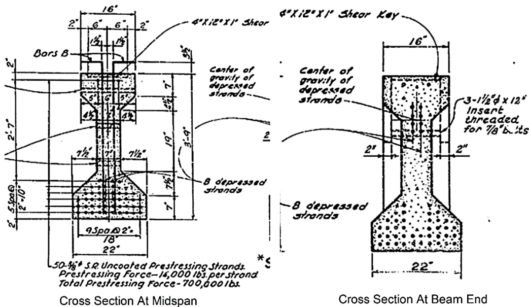
Figure 3. Cross Section of a Beam (Virginia Department of Highways, 1957)
