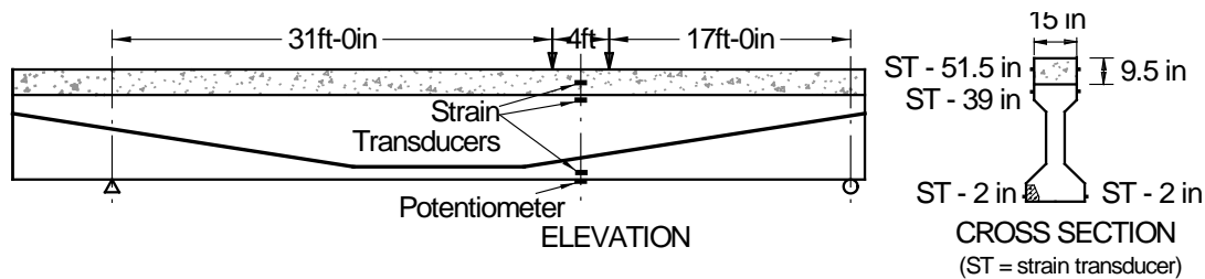
Figure 40. Test 6 Set-up and Instrumentation
