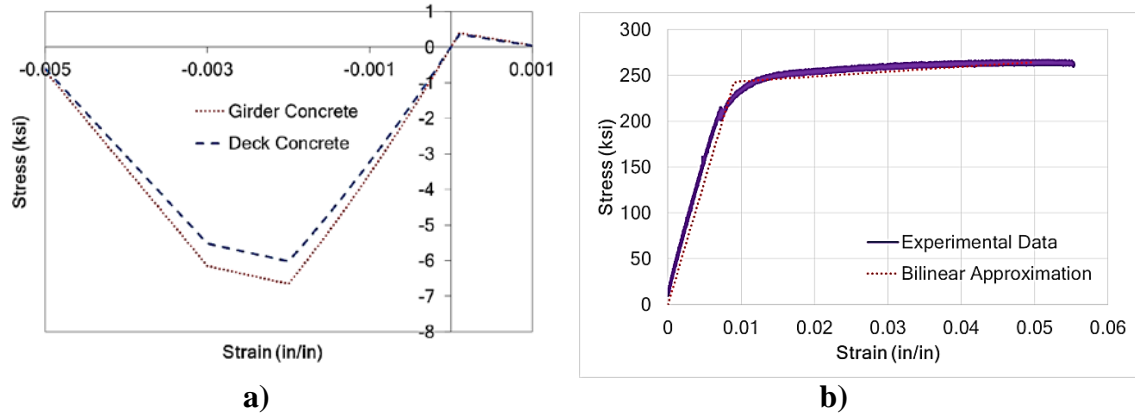
Figure 43. Calibrated Material Laws for Concrete and Steel: a) Hognestad Concrete Material Model (Hesham and Mohd, 1994) and b) Calibration of Tendon Material Model With Material Test Data
