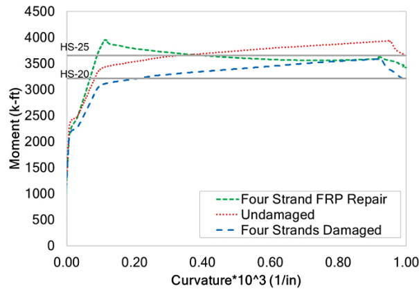
Figure 75. Moment-Curvature Response of Prototype Girder Investigating the Effect of an FRP Overlay on a Girder With 4 Strands Damaged
