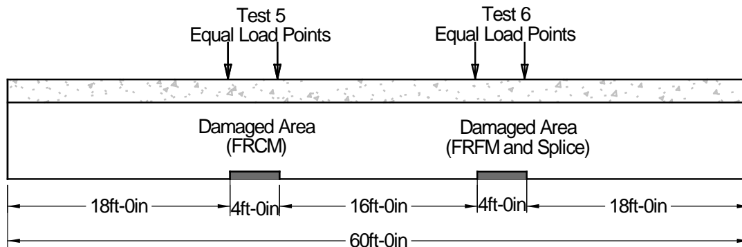
Figure 24. Beam D Damage Locations
