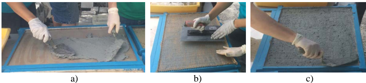
Figure 9. Specimen Preparation: a) First Layer of Mortar, b) Placing Mesh, c) Layer of Mortar (Sandwich)
