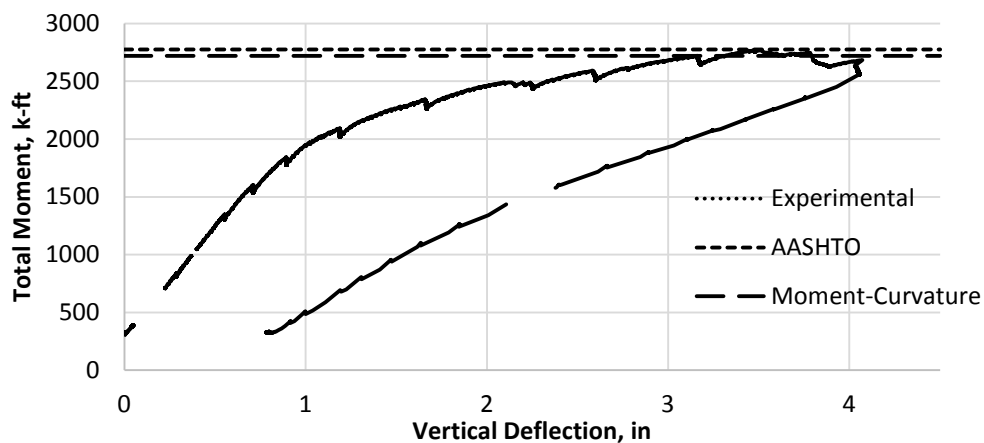
Figure 54. Test 2 Moment Versus Deflection Behavior
