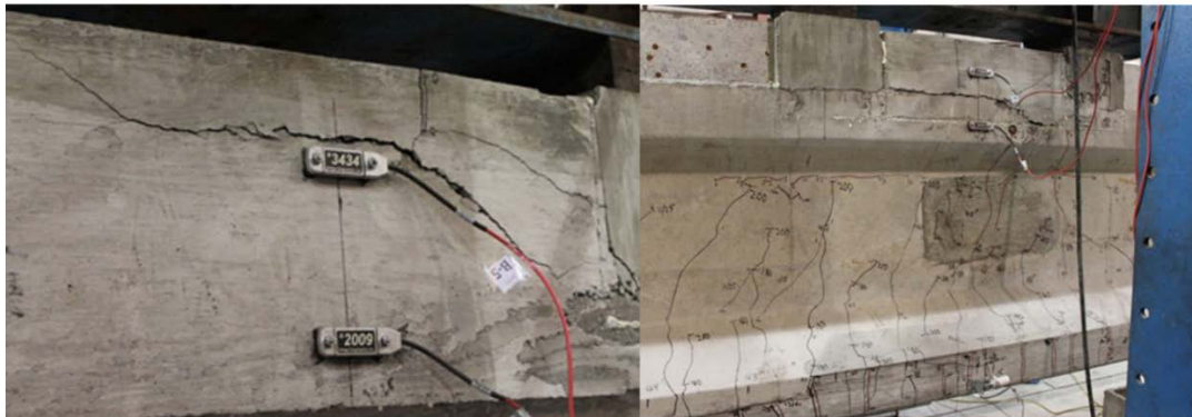
Figure 56. Test 4 Flexural Compression Failure in the Deck ( left ) and Cracking Pattern in Beam Below Load Point ( right )
