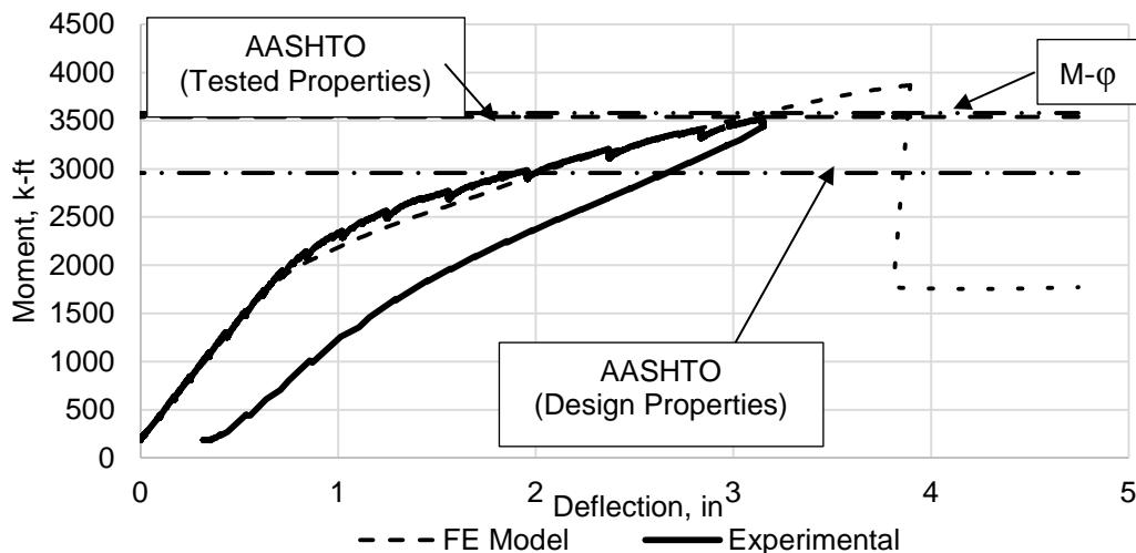
Figure 55. Test 3 Moment Deflection Behavior (M-φ = moment-curvature)
