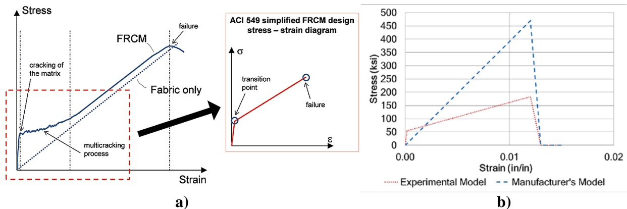
Figure 45. Uniaxial Material Laws for FRCM: a) Idealized Stress-Strain Curve (De Luca and Tumialan, 2014) and b) Alternative Stress-Strain Curves Employed in the Present Study
