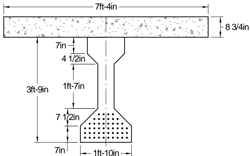
Figure 70. Prototype Girder Cross Section With Effective Bridge Deck
