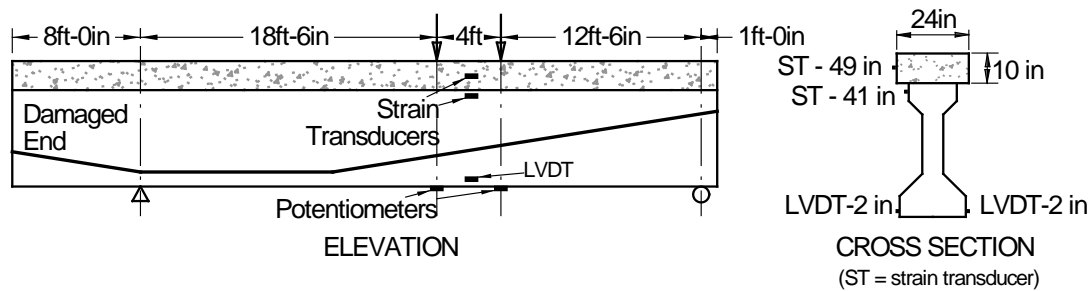
Figure 32. Test 1 Loading Arrangement and Instrumentation Layout
