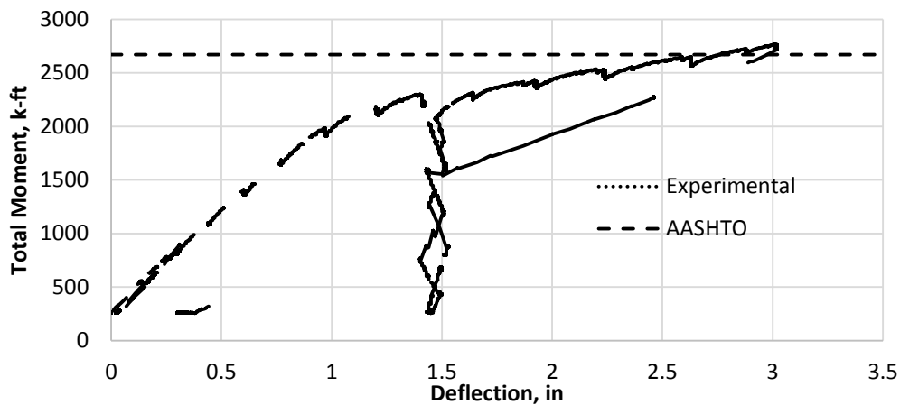
Figure 59. Test 5 Moment Versus Deflection Behavior
