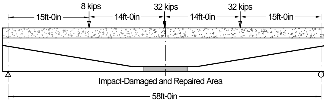
Figure 72. Prototype Girder Service Analysis Configuration With HS-25 Truck Loading
