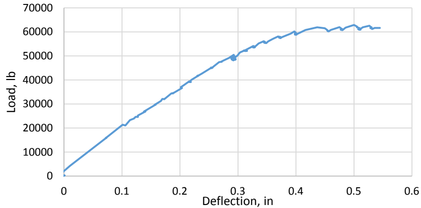
Figure 48. Second Test, Load versus Deflection Plot for Specimen 3 with Typical CFCC Reinforcement
