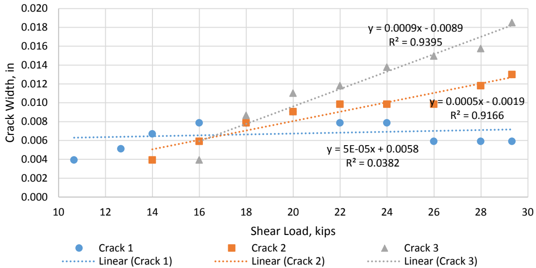
Figure 55. Crack Propagation for Specimen 4 with Two Layers of C-Grid Zip Tied Together
