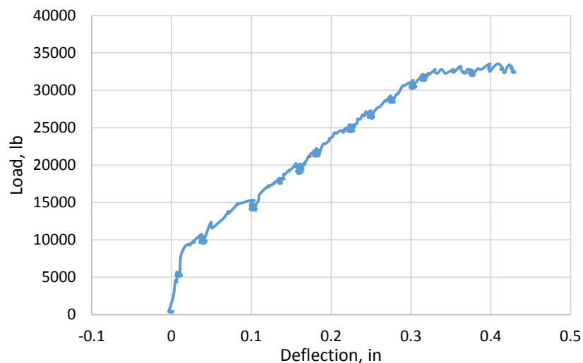
Figure 30. Load-Deflection Specimen 1 Minimum Steel
