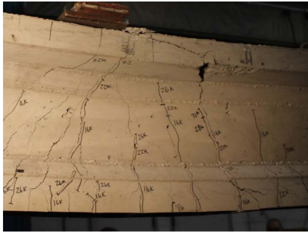
Figure 34. Top Flange Compression Failure of Specimen 1 Typical Steel Reinforcement
