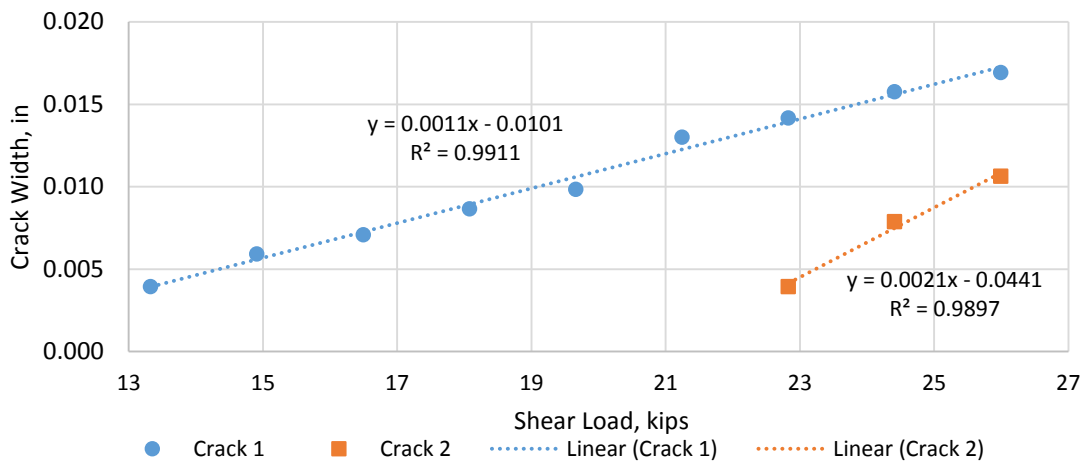
Figure 35. Measured Crack Width during Testing for Specimen 1 with Typical Steel Reinforcement
