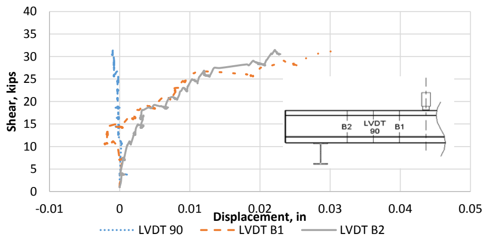
Figure 61. Vertical LVDT Displacement Measurements of Specimen 4 with Two Layers C-Grid Spaced Apart
