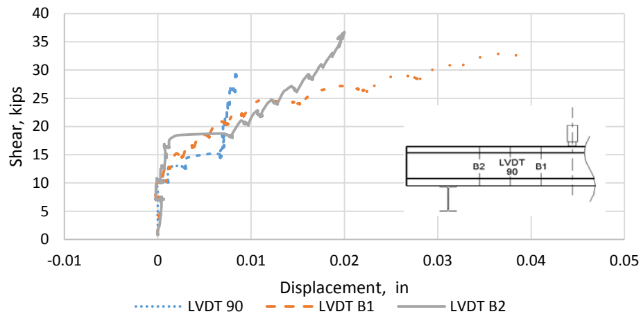
Figure 51. Vertical LVDT Displacement Measurements of Specimen 3 with Typical CFCC Reinforcement
