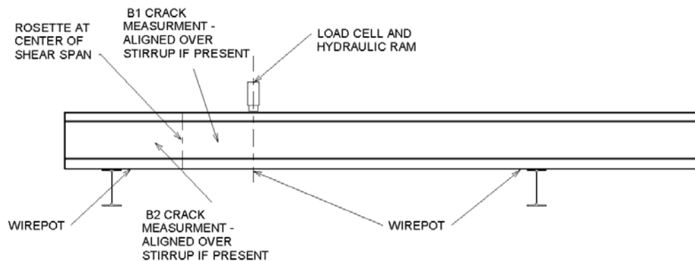
Figure 22. Full Instrumentation for Shear Testing
