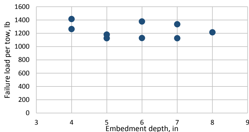
Figure 26. Failure Load versus Embedment Depth for C-Grid
