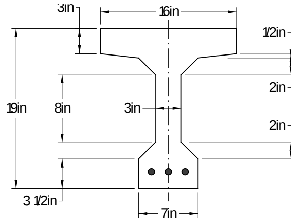
Figure 15. Beam Cross-Section
