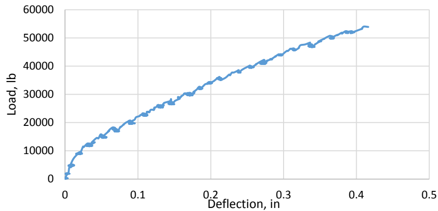
Figure 69. Load versus Deflection at Load Point for Specimen 5 with Typical NEFMAC Reinforcement
