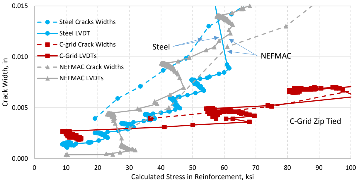
Figure 75. Calculated Reinforcement Stress versus Crack Width and LVDT Web Deformation
