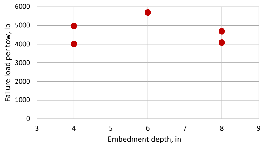
Figure 28. Failure Load versus Embedment Depth for NEFMAC Grid
