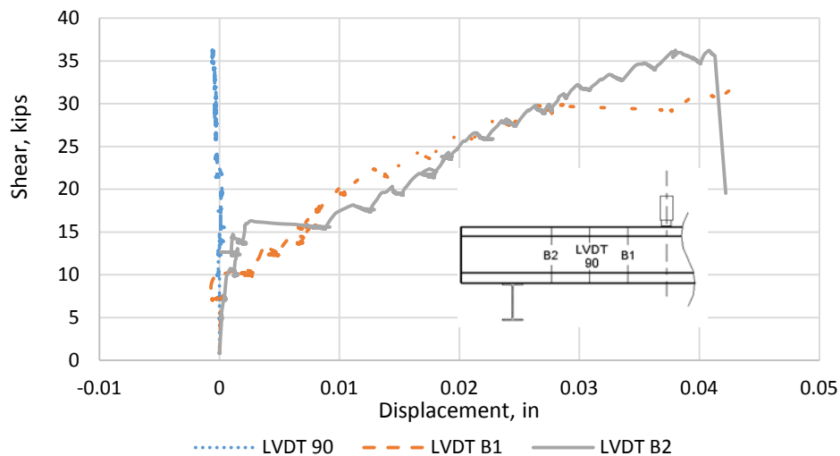
Figure 56. Vertical LVDT Displacement Measurements of Specimen 4 with Two Layers of C-Grid Zip Tied Together
