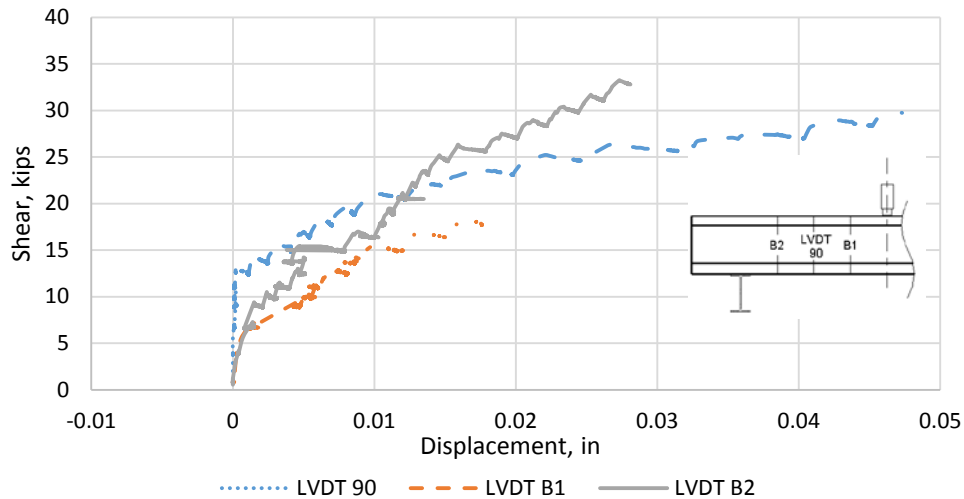
Figure 46. Vertical LVDT Displacements of Specimen 3 with Minimum CFCC Reinforcement
