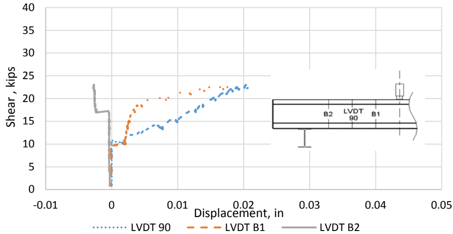
Figure 32. Vertical LVDT Displacement of Specimen 1 with Minimum Steel Reinforcement
