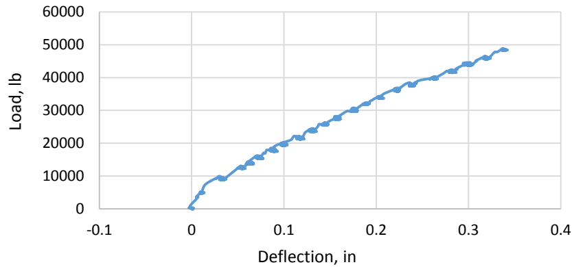
Figure 44. Load-Deflection Specimen 3 with Minimum CFCC Reinforcement
