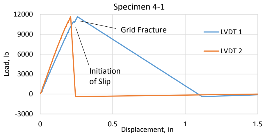
Figure 25. Typical Load versus Displacement Plot for C-Grid
