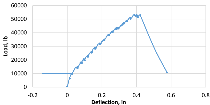
Figure 53. Load versus Deflection Plot of Specimen 4 with Two Layers of C-Grid Zip Tied Together
