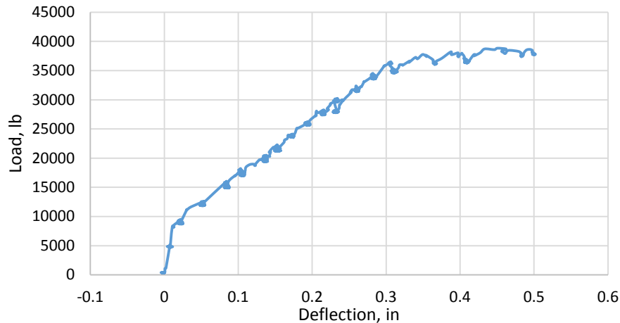
Figure 38. Load-Deflection Specimen 2 Minimum C-Grid Reinforcement
