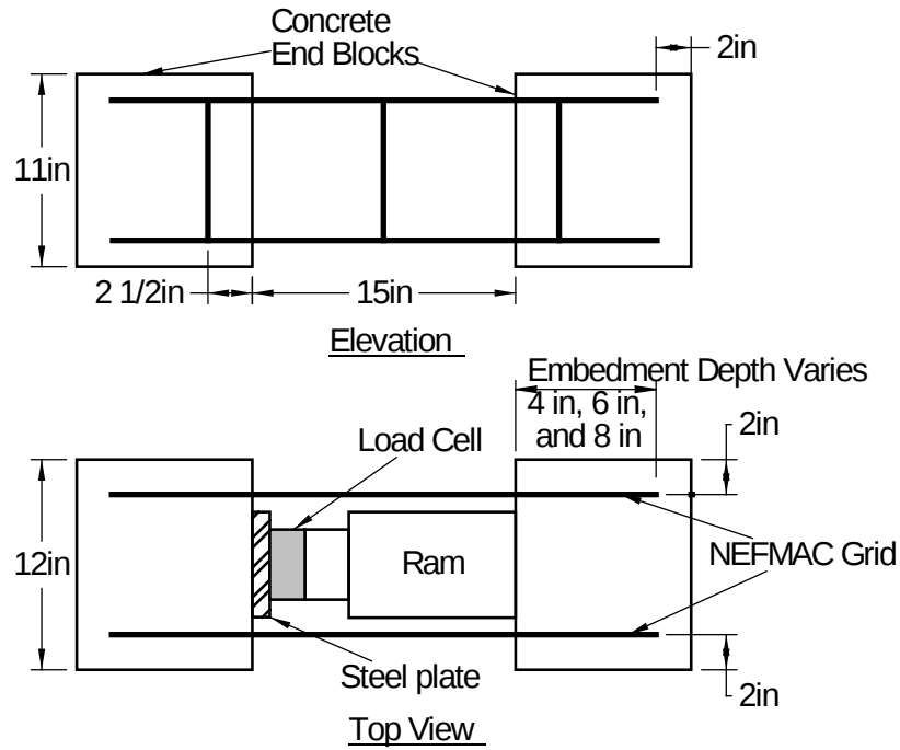
Figure 10. Typical Development Length Specimen for NEFMAC
