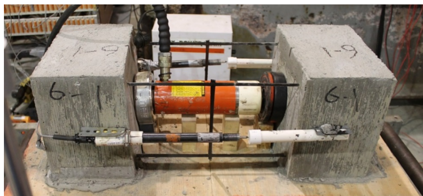
Figure 13. Typical NEFMAC Test Set Up
