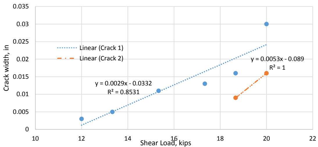
Figure 72. Crack Propagation of Specimen 5 with Typical NEFMAC Reinforcement
