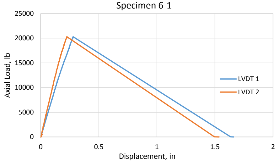
Figure 27. Typical Load versus Displacement Plot for NEFMAC Grid
