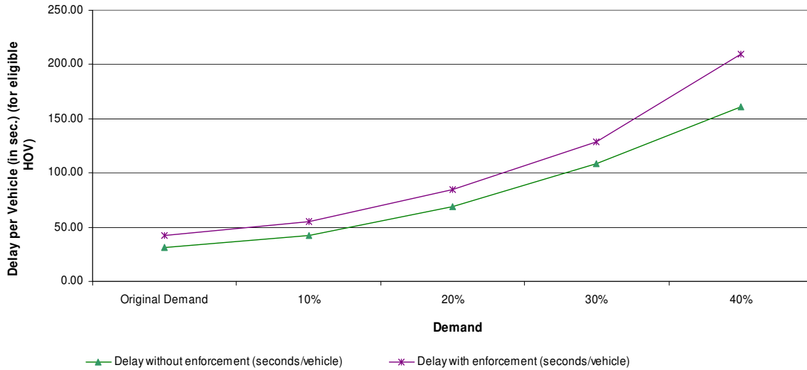
Figure 5. Delay Increase Corresponding to Demand Increase
