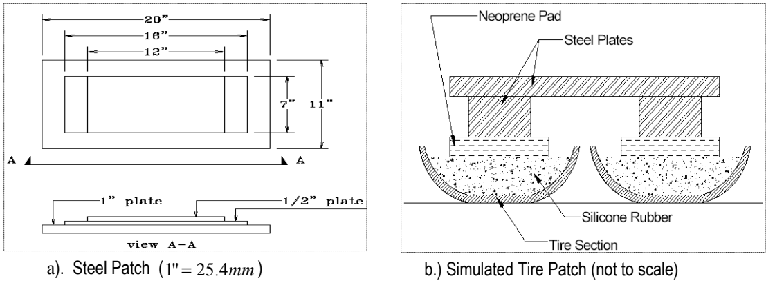
Figure 4 Loading patches used in laboratory tests
