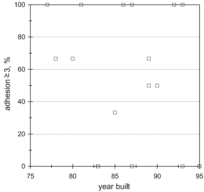
Figure 17. Percentage of Average Adhesion ≥ 3, Truss Bars
