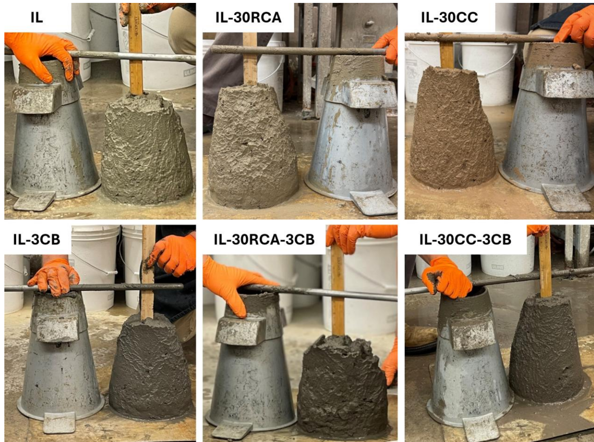
Consistency of Concrete Mixtures with and Without Carbon Black After Slump Test. CB = carbon black; CC = calcined clay; IL = Type IL Cement; RCA = reclaimed Class F coal ash.
