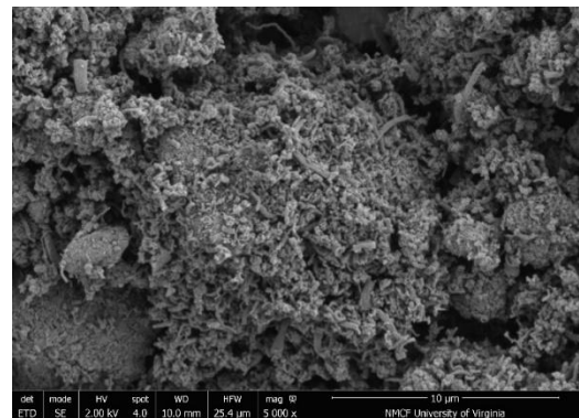
Scanning Electron Microscopy Image of Carbon Black (5,000x magnification)
